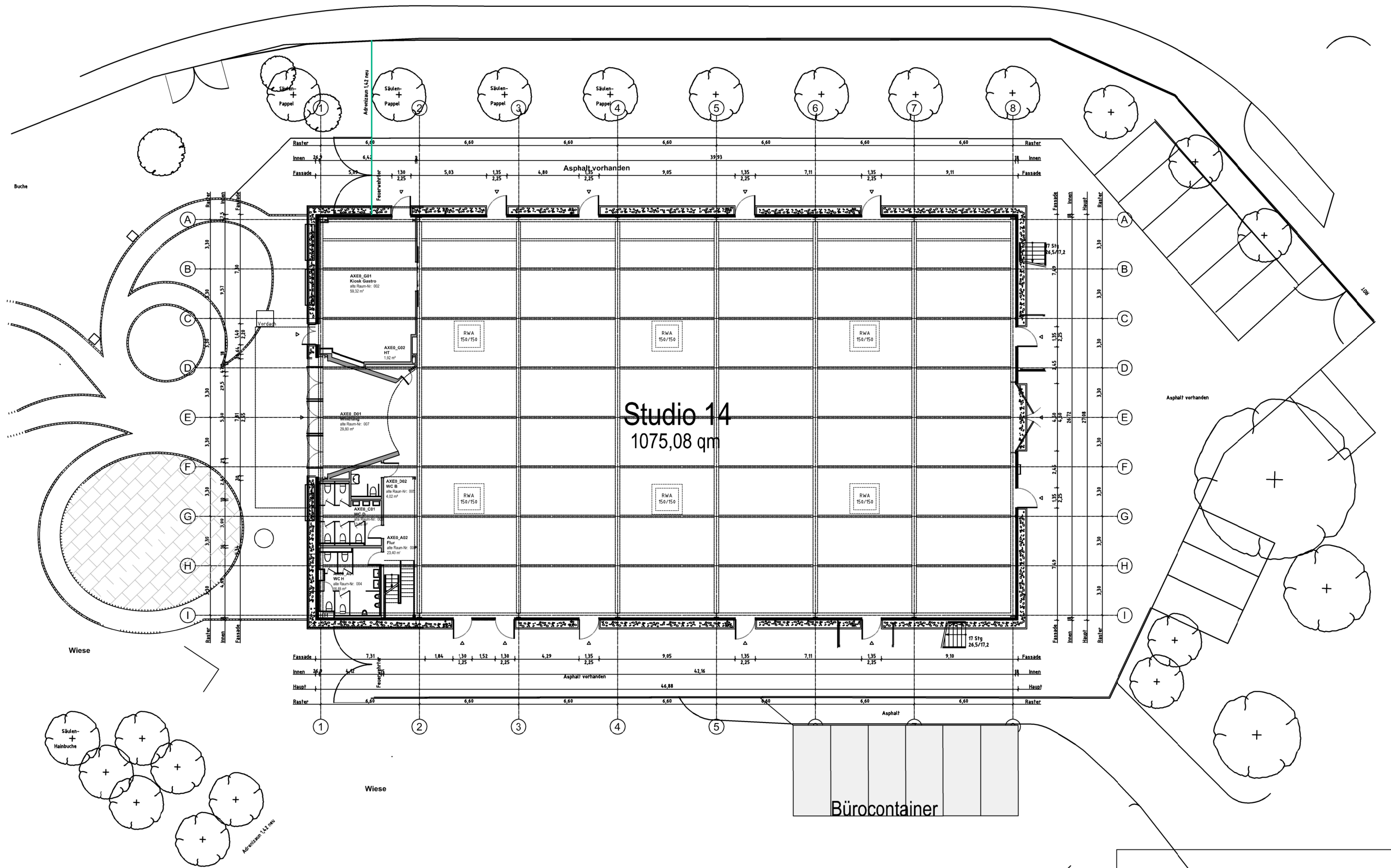
Studio 14 Grundriss
