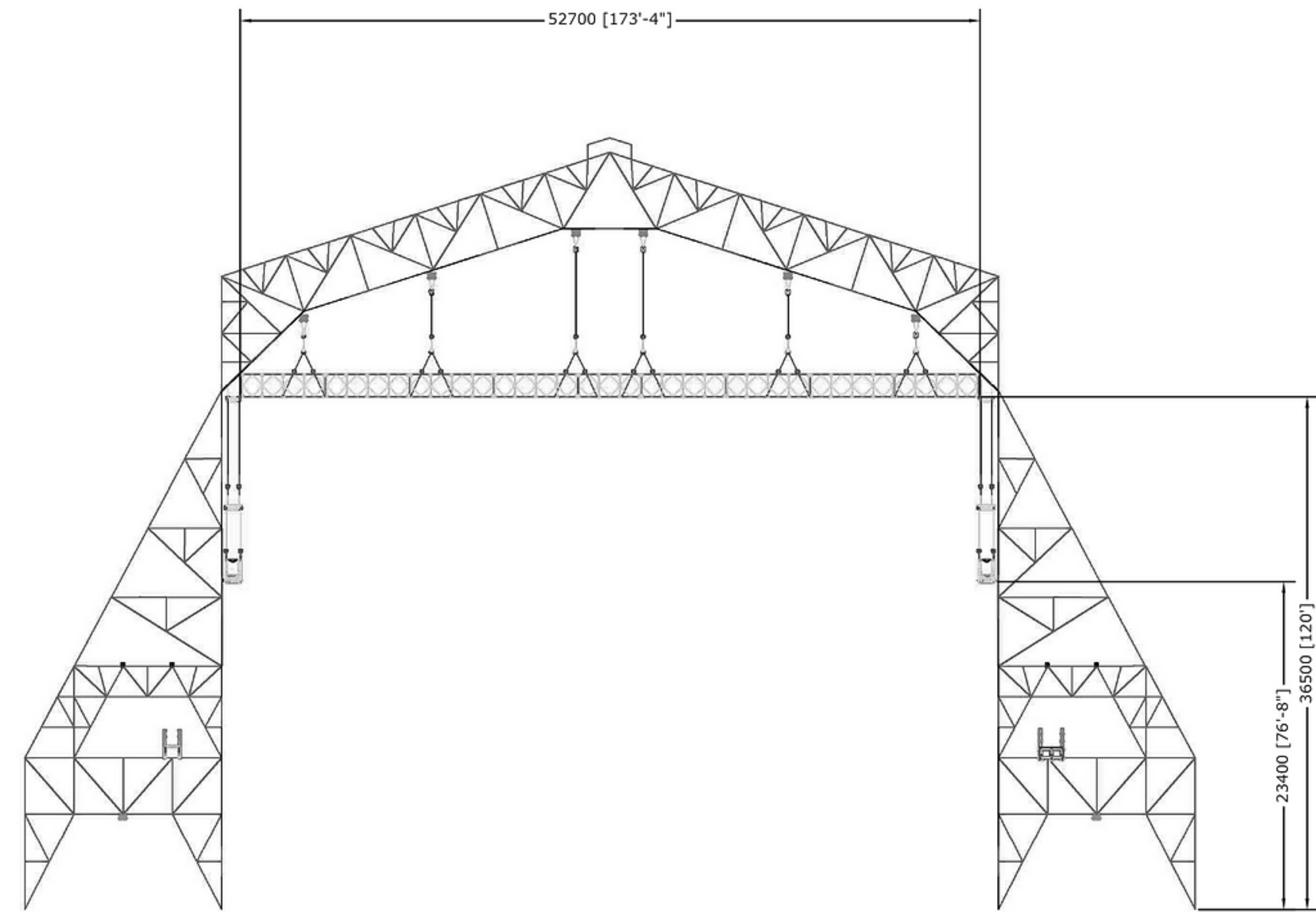
CLEARANCE WITH CROSS-STAGE CATWALK FLOWN OUT
