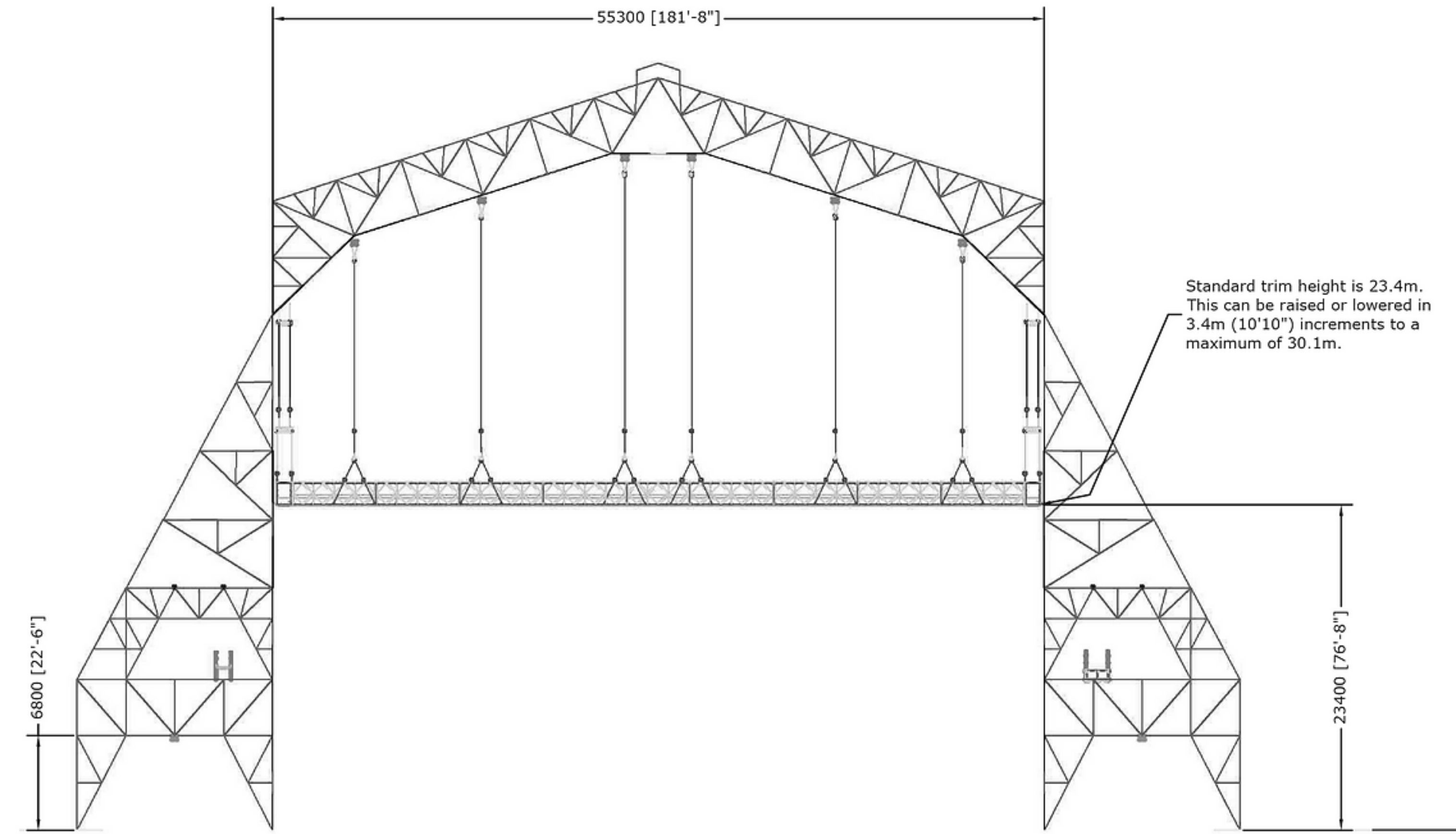
CLEARANCE WITH CATWALK IN THE STANDARD CONFIGURATION
