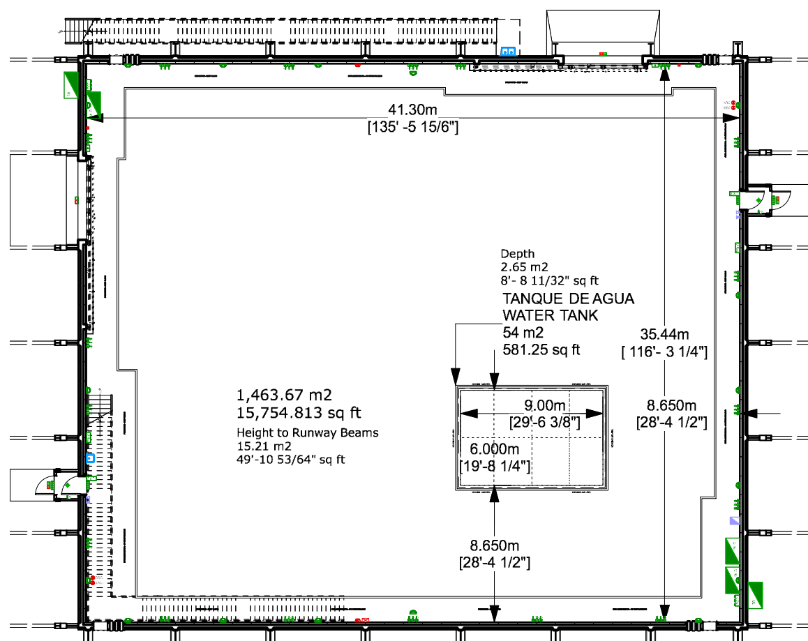
SS2 GROUND FLOOR
