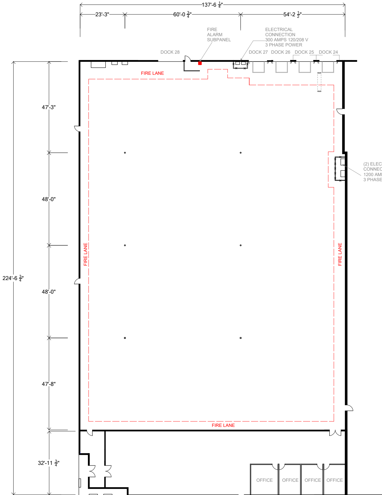
KEY PLAN
