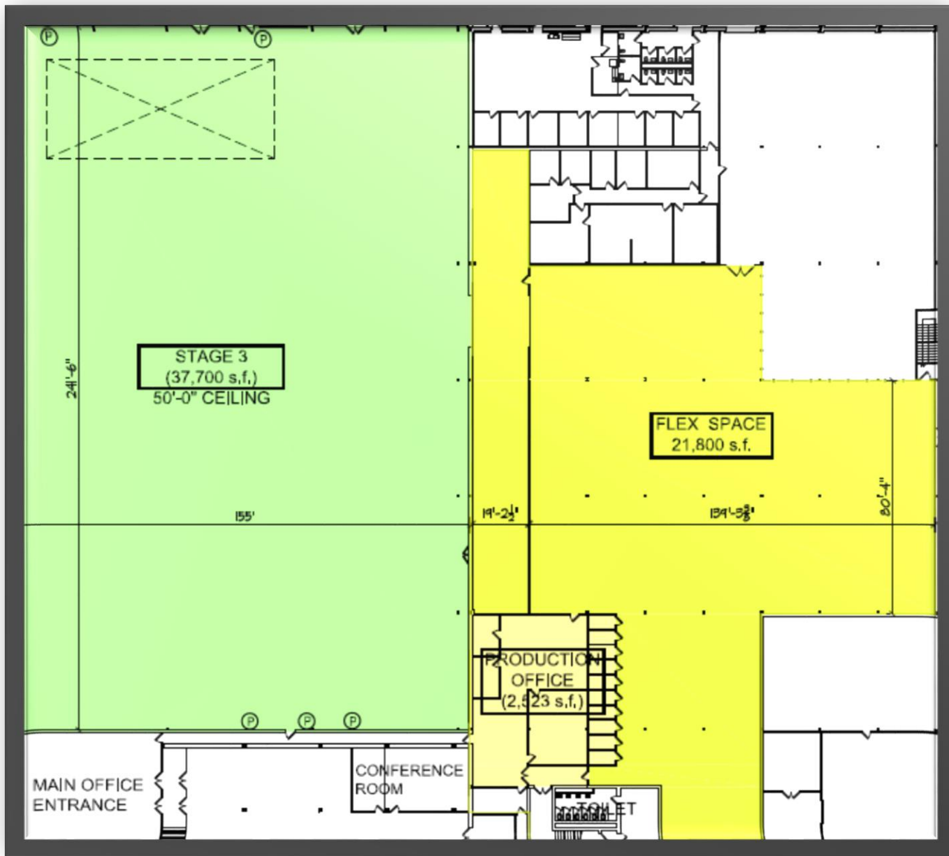
STAGE 3 FLOOR PLAN
