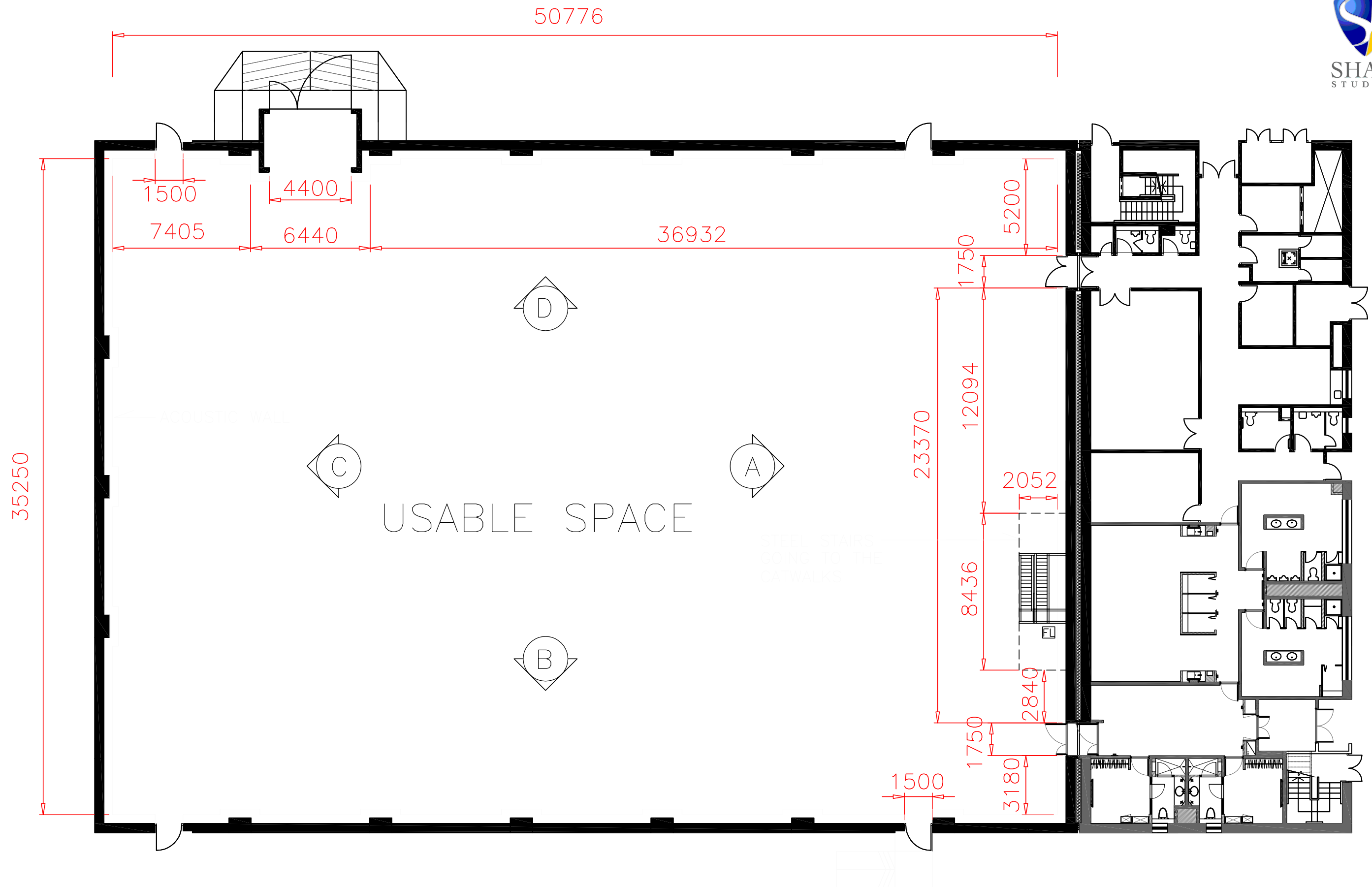
SOUND STAGE 1 PLAN MEASUREMENTS ARE IN MILLIMETERS (UNLESS SPECIFIED) SCALE 1:200 ON A3
