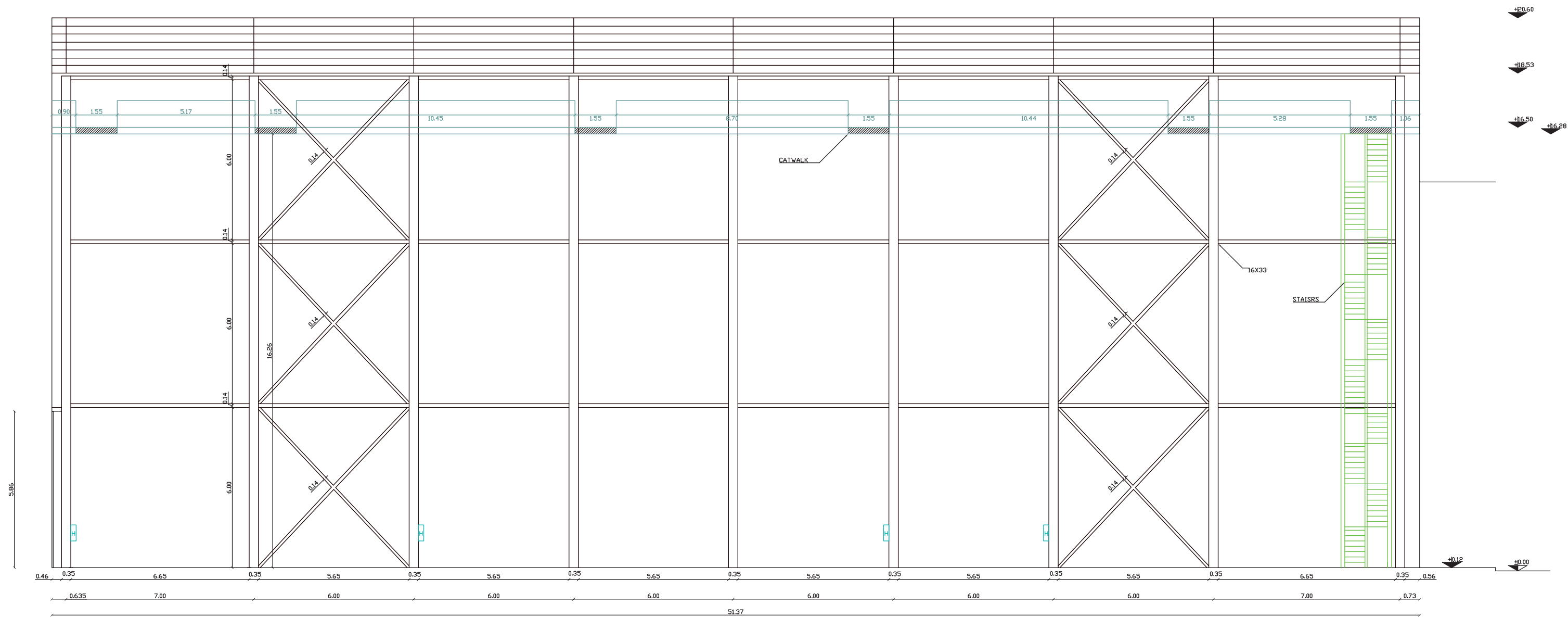
STAGE 8B LONGITUDINAL SECTION WIDTH = 14.41 LENGHT= 51.23 AREA =2121.94 SQM HEIGHT GANGWAY =16.00 M
