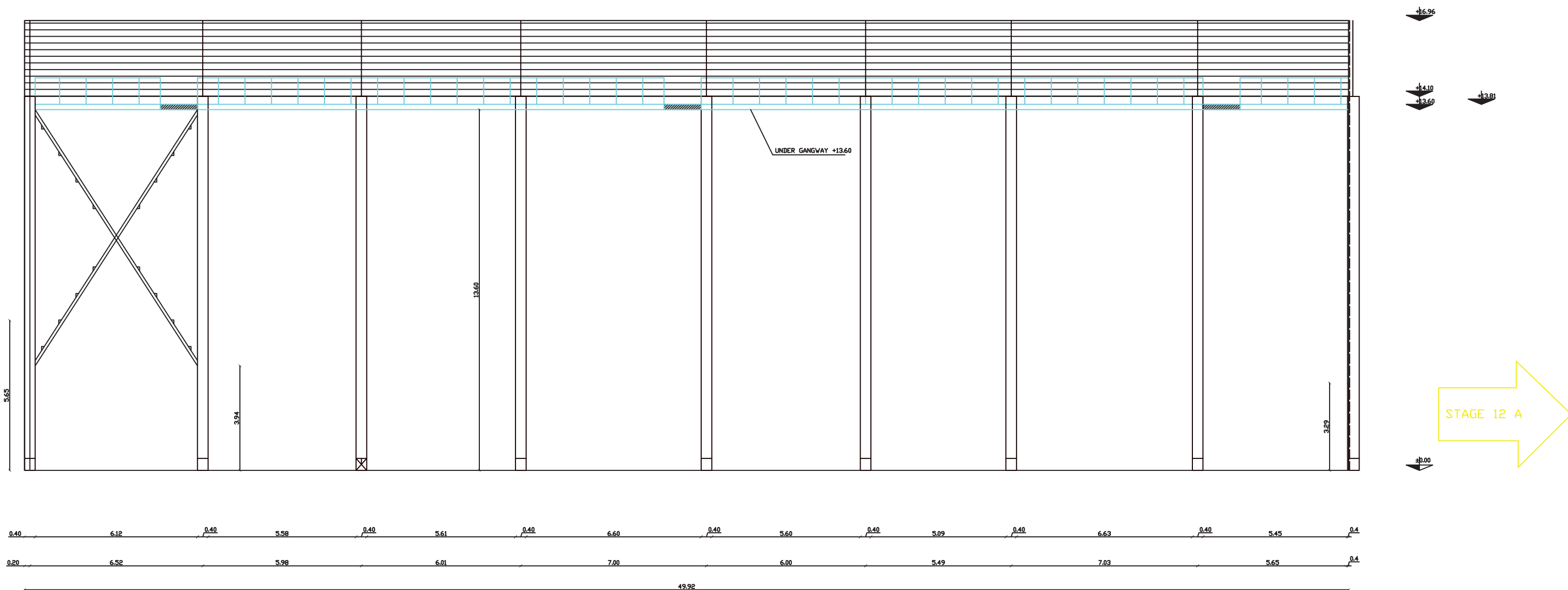
STAGE 12 B LONGITUDINAL SECTION
