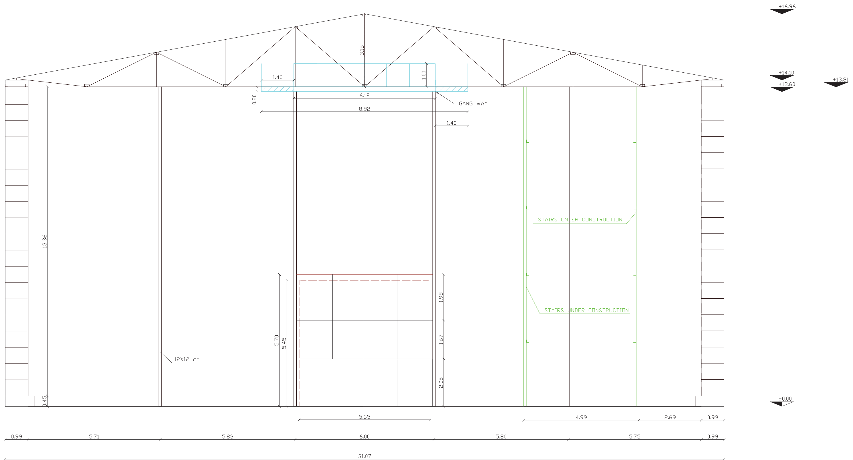
STAGE 12 B CROSS SECTION
