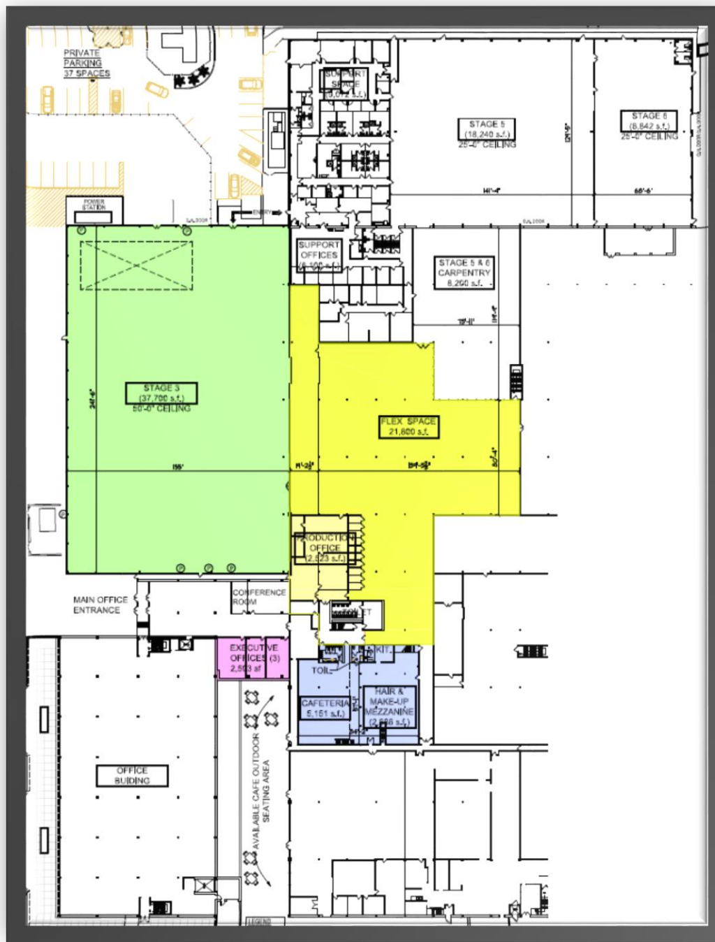
STAGE 3 FLOOR PLAN
